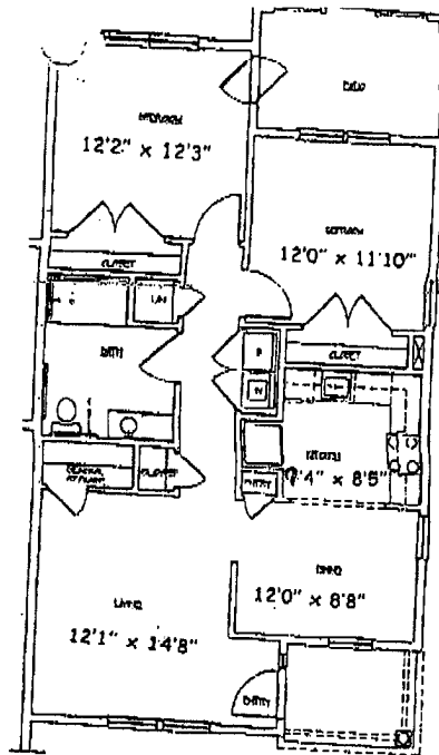
II FIRST FLOOR TWO BEDROOM TYPICAL UNIT
