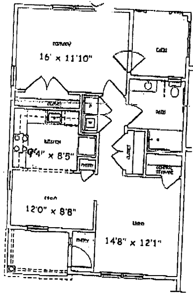
I FIRST FLOOR ONE BEDROOM TYPICAL UNIT
