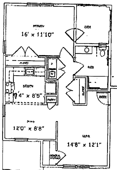
IV SECOND FLOOR ONE BEDROOM TYPICAL UNIT
