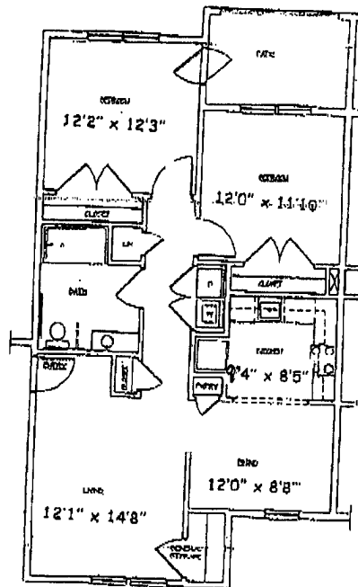
V SECOND FLOOR TWO BEDROOM TYPICAL UNIT
