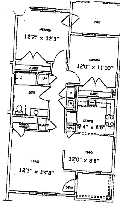
II FIRST FLOOR TWO BEDROOM TYPICAL UNIT
